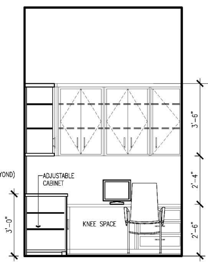
15 OFFICE Scale : 3/8"=1'
