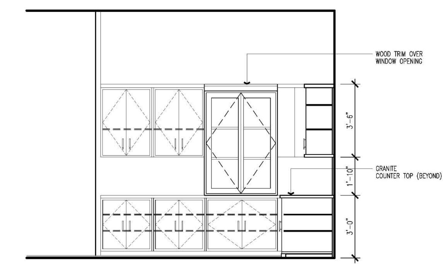
13 KITCHEN Scale : 3/8"=1'
