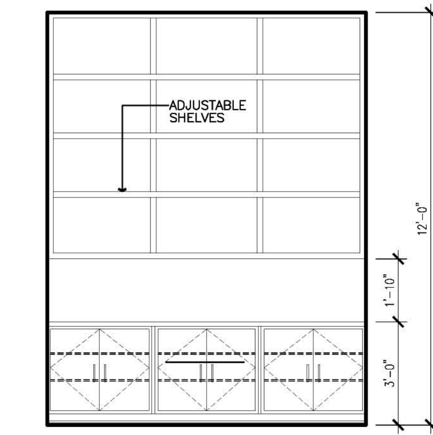
18 PANTRY Scale : 3/8"=1'
