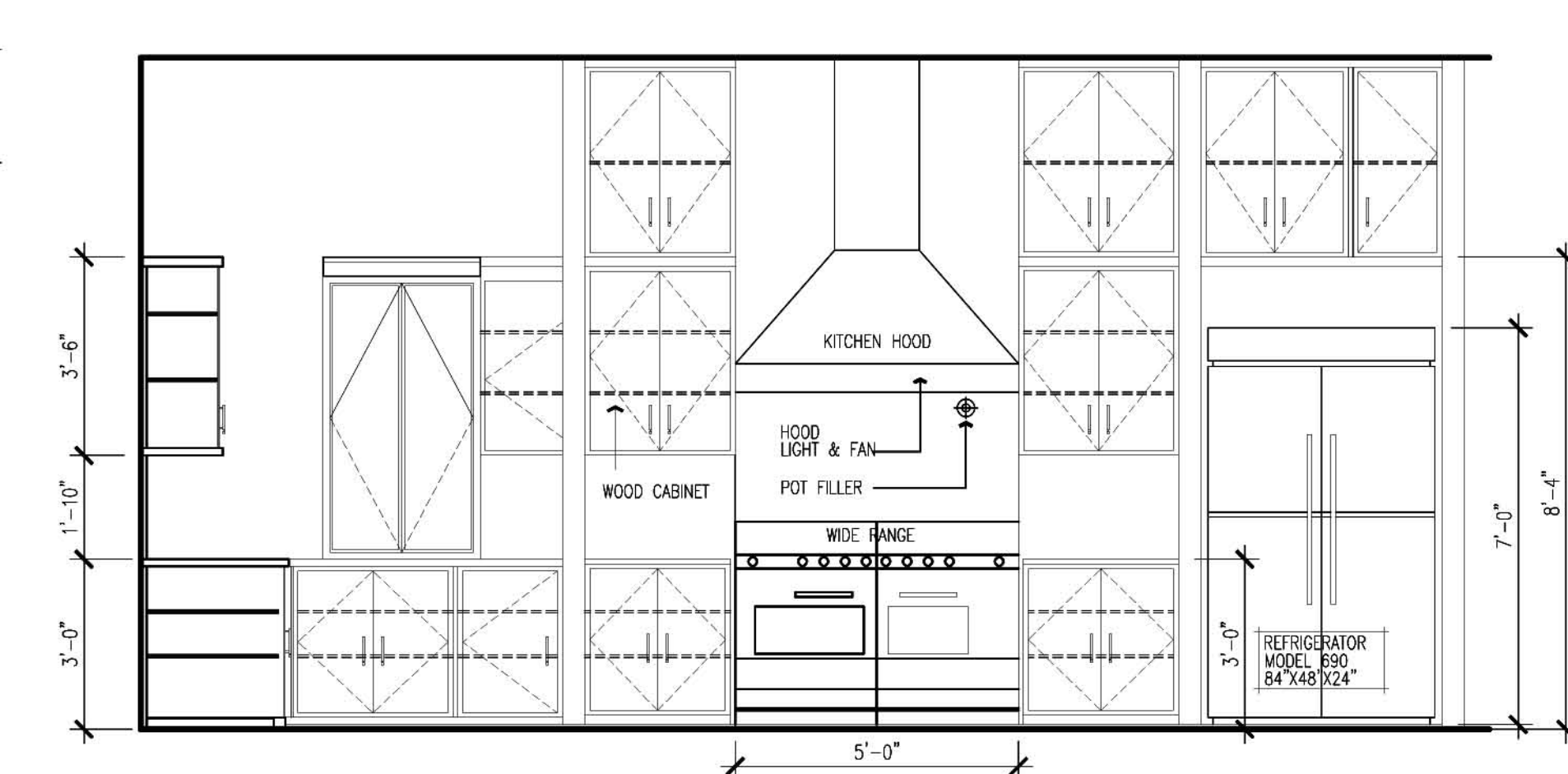
12 KITCHEN Scale : 3/8"=1'
