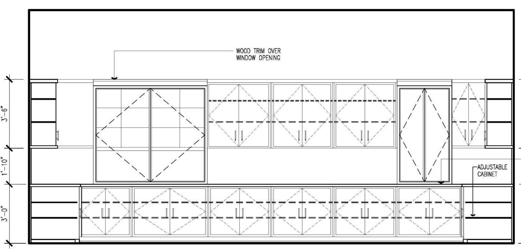
14 KITCHEN Scale : 3/8"=1'
