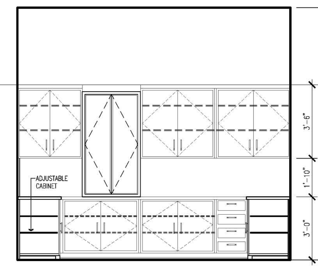
16 OFFICE Scale : 3/8"=1'
