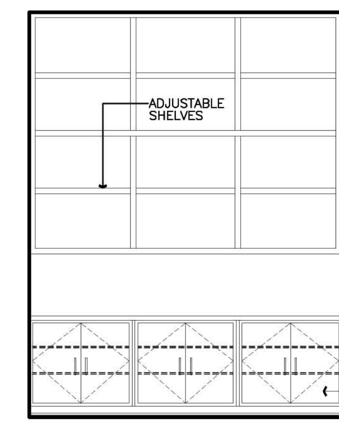
17 PANTRY Scale : 3/8"=1'
