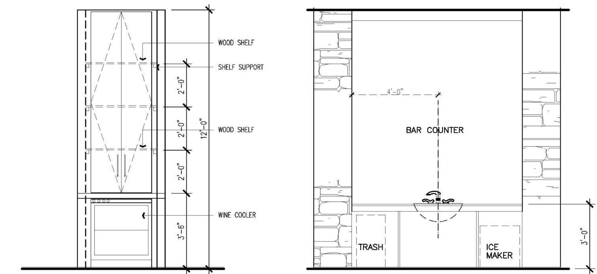
09 PANTRY Scale : 3/8"=1'
